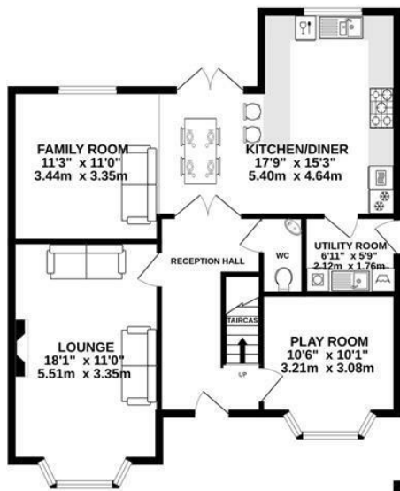
GROUND FLOOR 1125 sq.ft. (104.5 sq.m.) approx.
